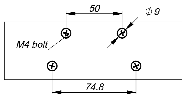
F 1:2 View without dispenser
